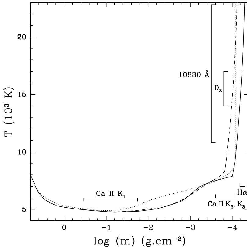
Fig. 2.— Temperature vs column mass distribution of the computed atmospheric models. The models shown were obtained with the microturbulent velocity of Fontenla et al. (1991) (dashed line), and with a value of 5 km/s in the region of formation of the lines (solid line, see text). The plage model P (Fontenla et al. 1993) is displayed for reference (dotted line). Also shown are the heights of formation of the different lines we used to build the models. The He I 584 line is formed at temperatures between 2.4 \times 10^4 and 3.4 \times 10^4 K, and the He II 304 line is formed between 9.5 \times 10^4 and 1. \times 10^5 K.
