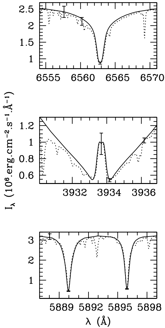
Fig. 3.— Observed (dashed line) and computed (solid line) profiles for H \alpha and the Ca II K and Na D lines. The bars indicate the r.m.s. of the averaged profiles (see text) and point out the variability between pixels.
