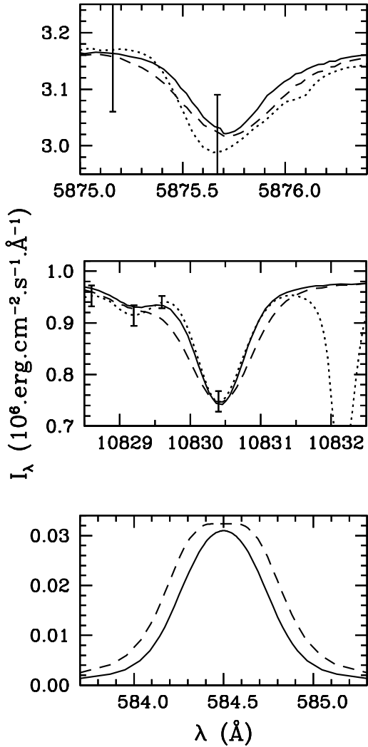
Fig. 4.— Comparison between observed and computed profiles of three Helium lines. Dotted line: observed. Dashed line: computed profiles (convolved with instrumental response) for the model adopting the microturbulence of Fontenla et al. (1991). Full line: same as dashed, for our standard model where microturbulence has been reduced (see text). In the upper and middle panel, bars indicate the r.m.s. of the averaged profiles and point out the variability between pixels. For the shallow D_3 line (maximum central depth \approx 5\% ) the variability is very large and the bars are clipped at the limits of the plot.
