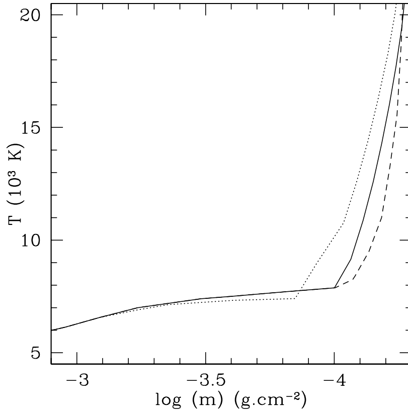
Fig. 7.— Temperature vs column mass distribution of the atmospheric models obtained for different values of the He abundance, in the region where they differ. Solid line: [\text{He}] = 0.1 , our standard model. Dotted line: [\text{He}] = 0.07 . Dashed line: [\text{He}] = 0.15 .
